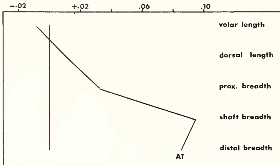
TEXT-FIG. 3. Ratiodiagram (Simpson 1941) comparing phalanx 1 of Sinohippus from Altan Teeli (AT) with Hypohippus (standard) from the Lower Clarendonian, Cherry County, Nebraska.
